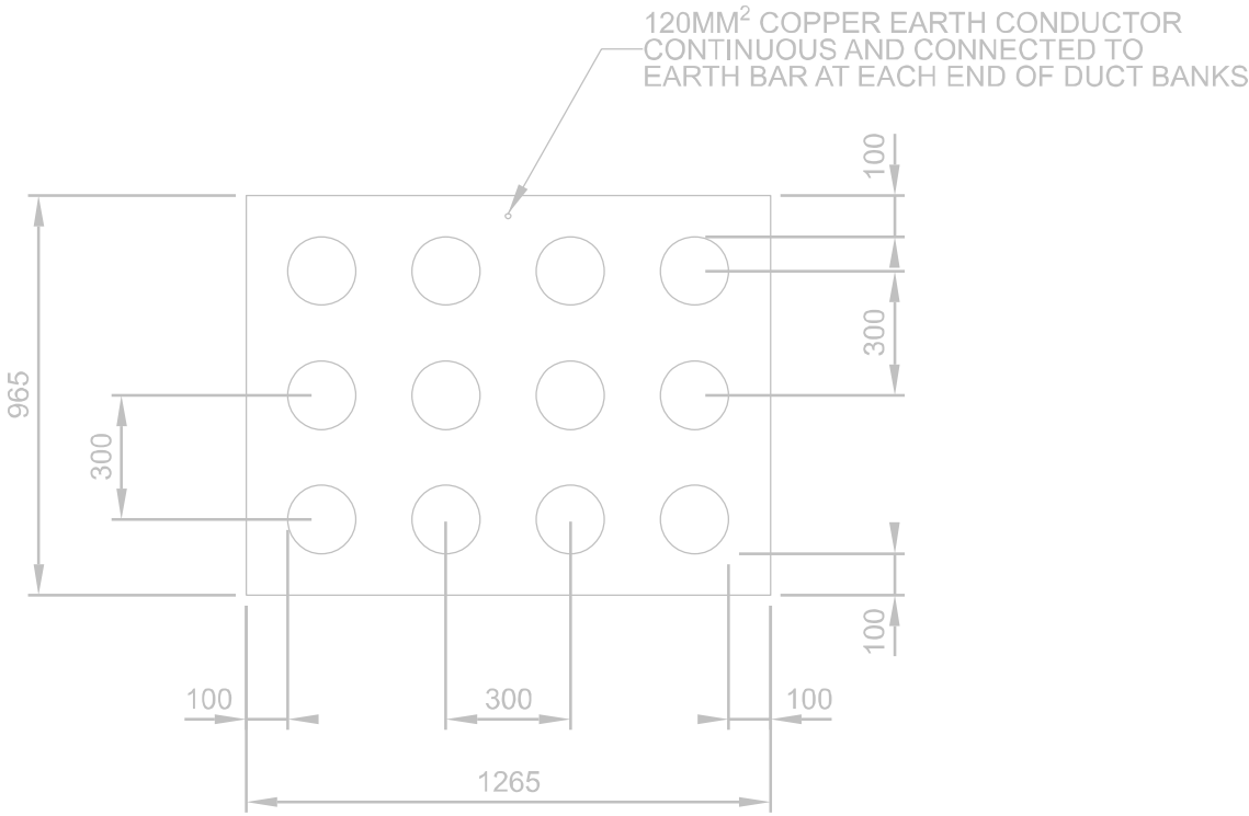
WSW31-EDUCT-0001, WSW31-EDUCT-0002 HD UPVC PIPE ENCASED IN CONCRETE
