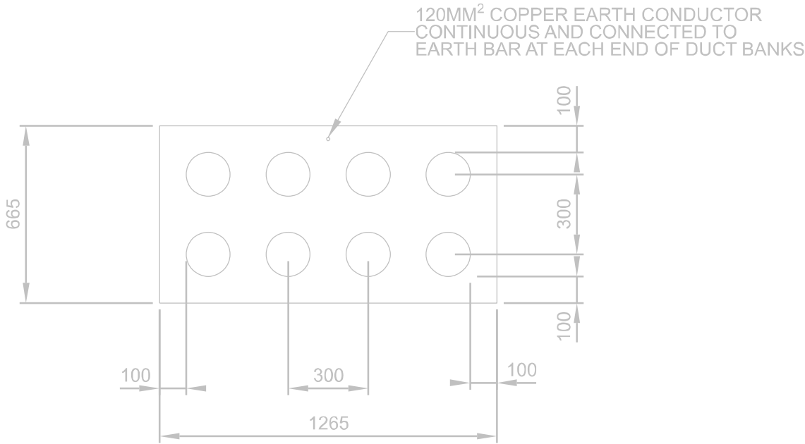
WSW31-EDUCT-0004, WSW31-EDUCT-0005, WSW31-EDUCT-0006, WSW31-EDUCT-0007, WSW31-EDUCT-0008 HD UPVC PIPE ENCASED IN CONCRETE
