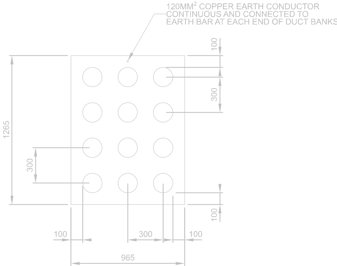
WSW31-EDUCT-0003 HD UPVC PIPE ENCASED IN CONCRETE
