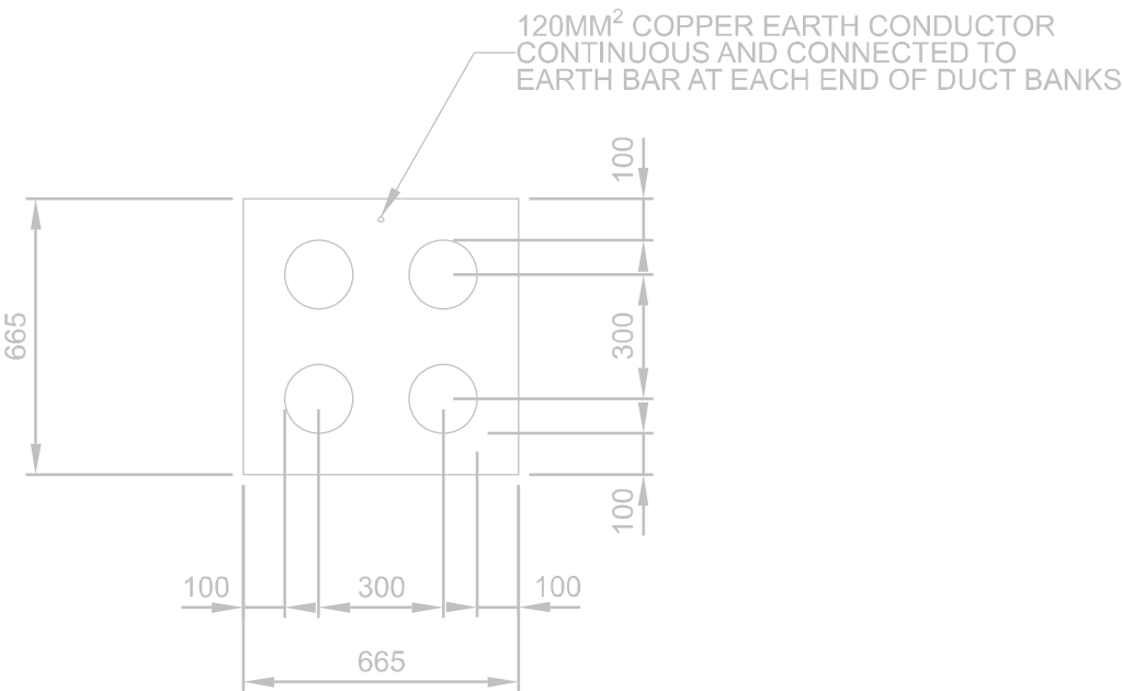
WSW31-EDUCT-0009, WSW31-EDUCT-0010, WST02-EDUCT-0001 HD UPVC PIPE ENCASED IN CONCRETE
