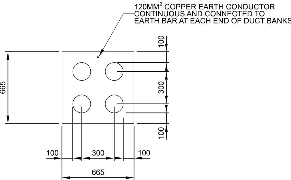
WST02-EDUCT-0001, WST02-EDUCT-0002, WST02-EDUCT-0003 HD UPVC PIPE ENCASED IN CONCRETE
